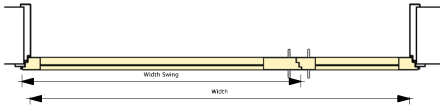
PLAN DIMENSIONS DOUBLE DOORS
